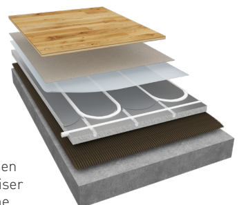
LK CombiBoard EPS 14/18/30/50/70
