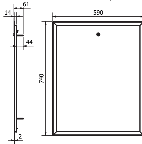
LK Ramme/luke GV 550, INB
