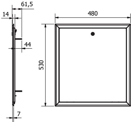
LK Ramme/luke M60n, INB
